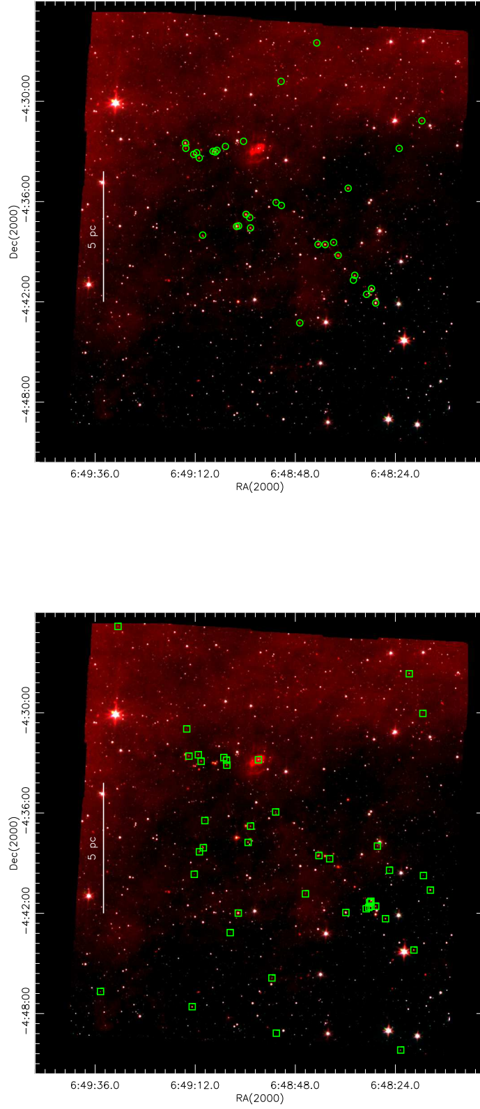
Fig. 6.— Top: the distribution of protostars. Bottom: the distribution of young stars with disks. The background image is the combined IRAC 3.6 (blue), 4.5 (green) and 8 \mu\text{m} (red) image.
